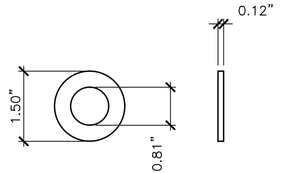
WASHER X2
