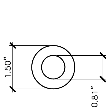
WASHER X2
