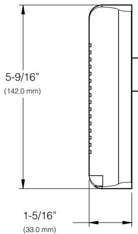
914C Interior
