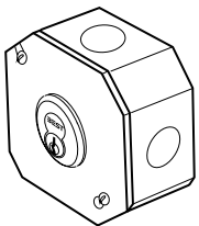
OC1 Standard octagon 3 1/2" x 3 1/2" x 1 5/8"
