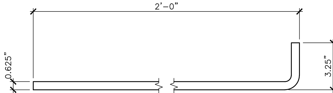
FRONT
