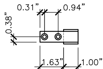
FRONT SIDE LOCKING BRACKET
