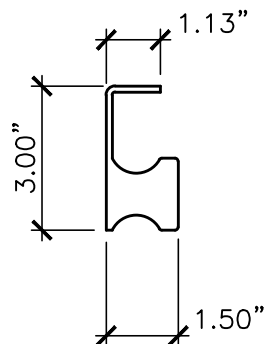
SIDE
