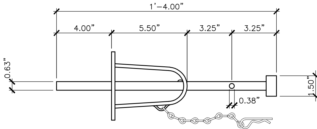
FRONT
