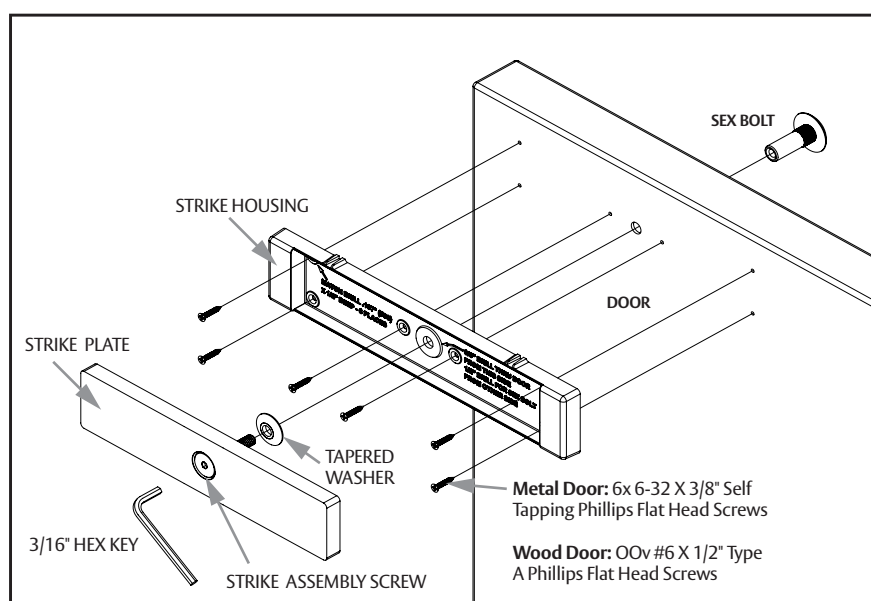
Diagram 13 Securing the plate assembly to the door
