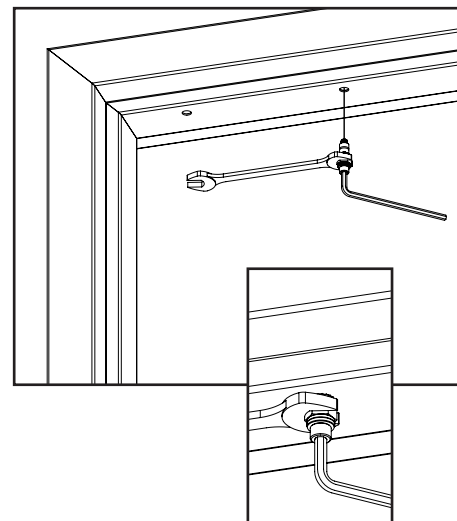
Diagram 8 Installing the blind nuts
