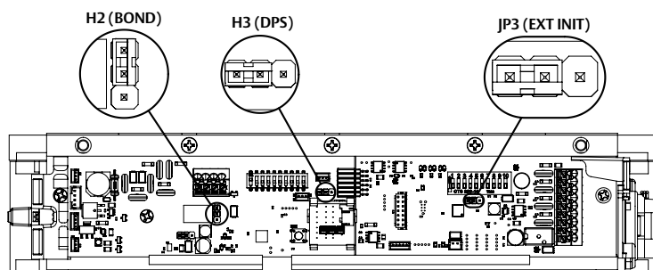
Diagram 29 Jumper Locations
