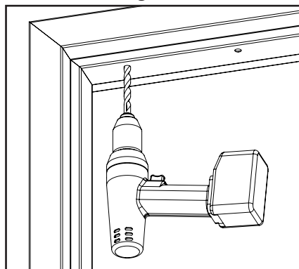
Diagram 7 Drilling the bracket mounting holes
