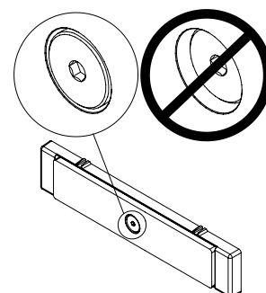
Diagram 15 Strike assembly installed – inside door
