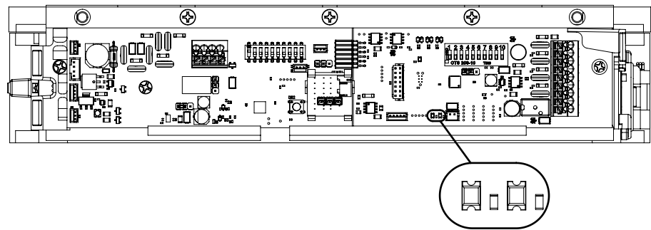
Diagram 31 LED location
