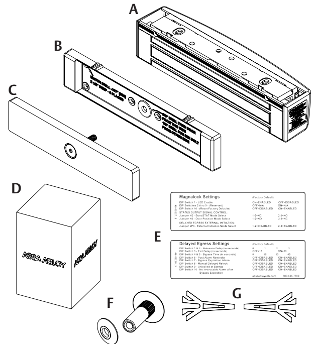
Diagram 1 Product Components
