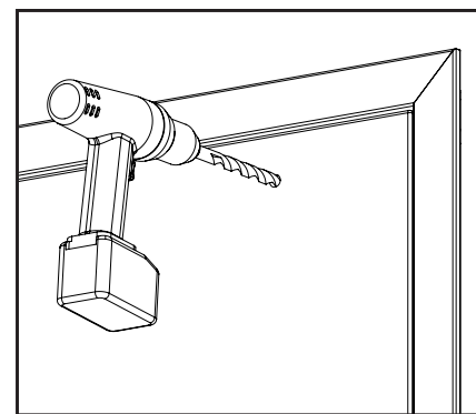
Diagram 12 Drilling the sex bolt hole from the outside
