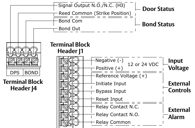
Diagram 25 Terminal pin-out diagram
