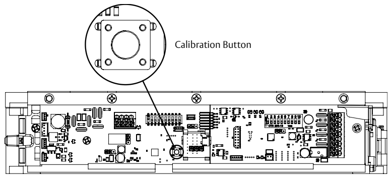
Diagram 34 Calibration button
