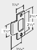
005075-000 T-strike, square corner
