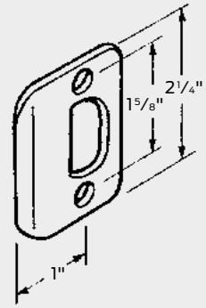
Q001-048 Full lip, \frac{1}{4} " radius corner
