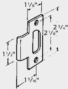
Q001-046 T-strike square corner
