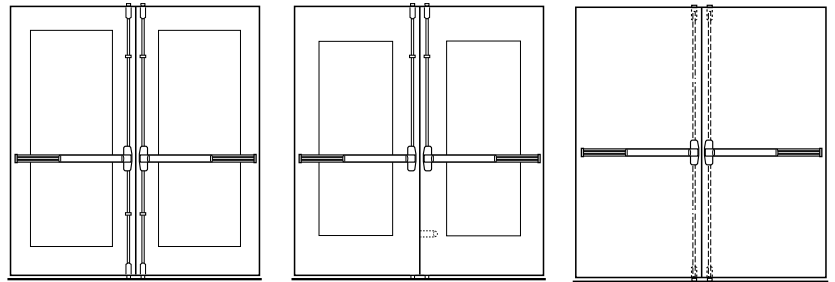
Two surface mounted vertical rod devices—same direction (do not use with overlapping astragal)
