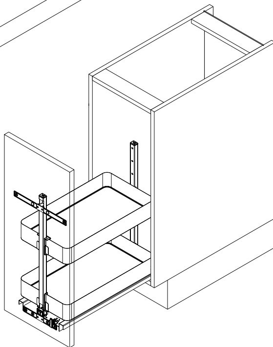
Frameless Cabinets
