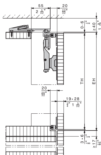
Door centring with magnetic centring elements.
