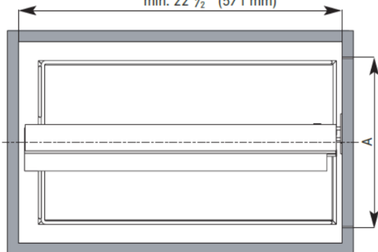
FRAMED CABINET
