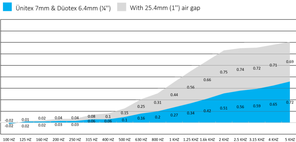
Absorption coefficient spectrum (ASTM C423)
