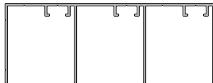
011188 Binario superiore 3vie Upper rail 3ways
