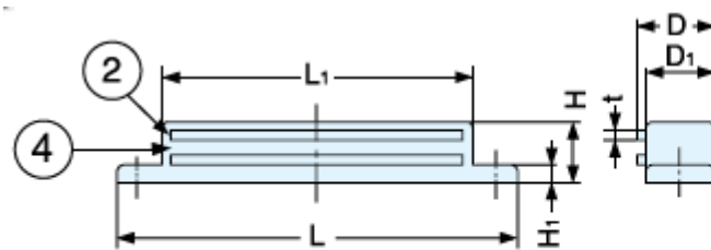
Double plate type
