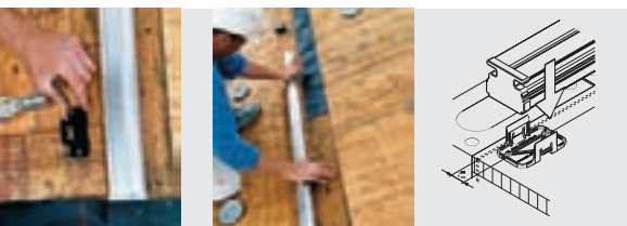
HAWA-Adapto assembly: nail plastic clips to shuttering, clip on profile, pour concrete – job done.
