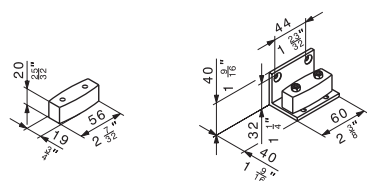
Point-fixing floor guides.
