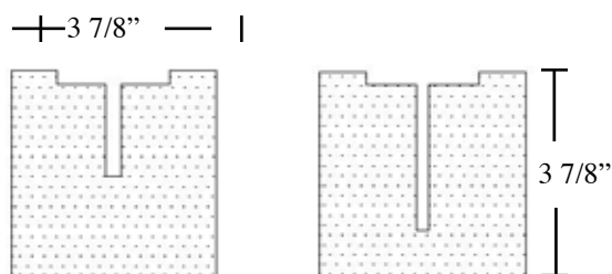
Face Plate for 2" x 2" T EHFP-0202
