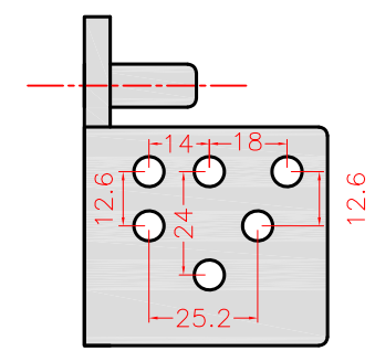
X bracket (4:1)
