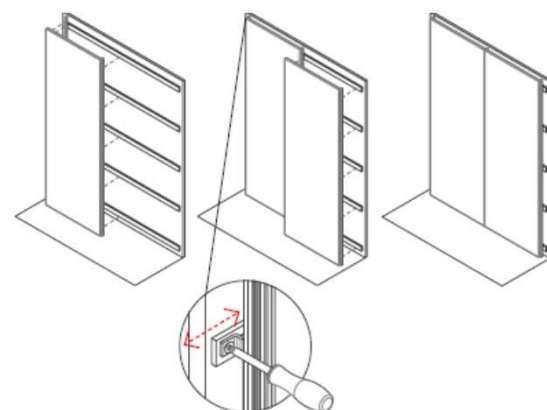
Installation of profiles on wall
