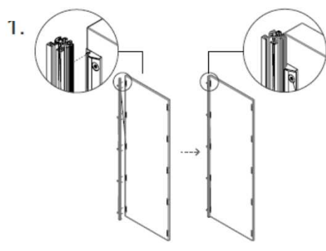
Installation of wall panels onto the profiles and ajustements.
