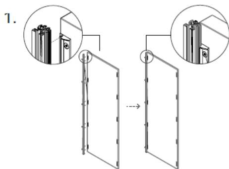
Installation of wall panels onto the profiles and adjustments.
