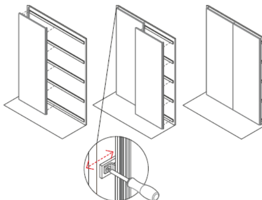
Preparation of wall panels with clips
