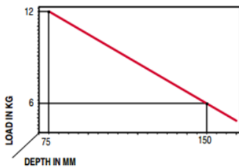
COMBINATION SHELF LOAD AND SHELF DEPTH (The figures refer to 1 shelf support)
