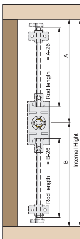
Installation dimensions
