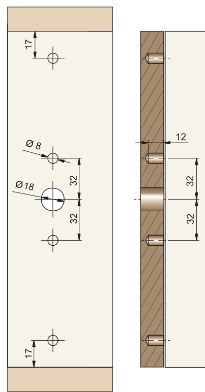
Drilling template to fasten with dowels
