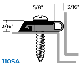
110SA 110SDKB
