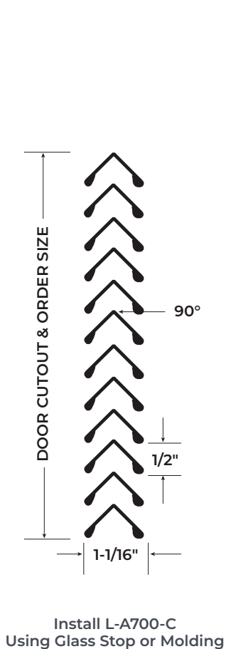
L-A700-C Undersized 1/4" for Clearance
