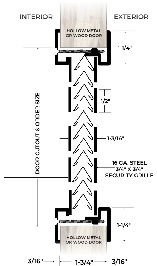
L-VRSG-3 Undersized 1/16" for Clearance
