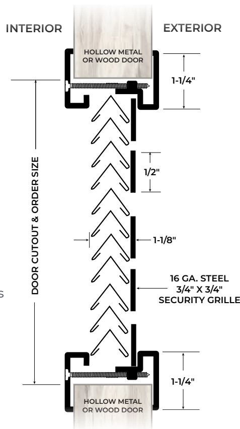
L-VRSG-2 Undersized 1/16" for Clearance
