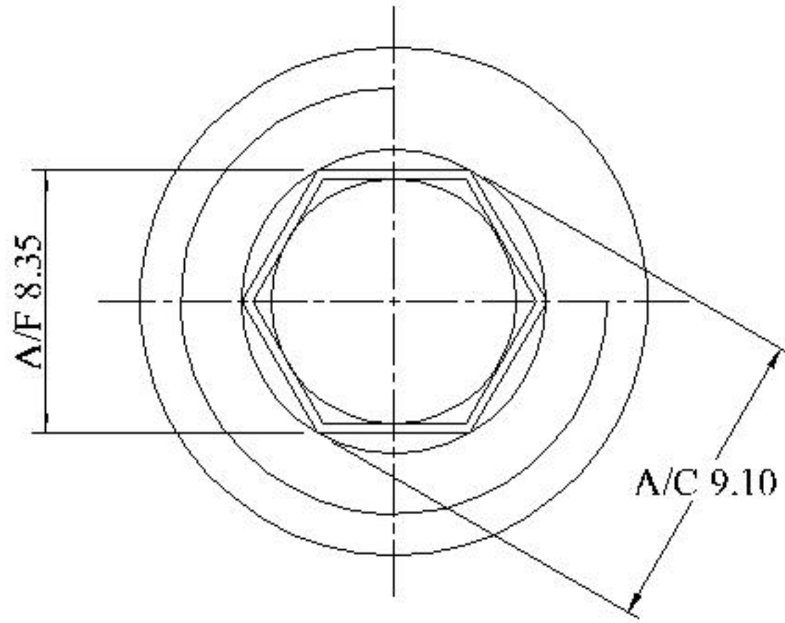
Dimensions for top of hex
