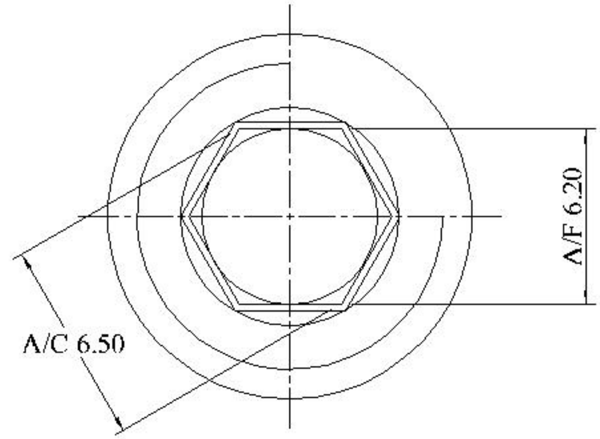
Dimensions for bottom of hex
