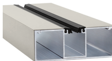
Sidelite Header
