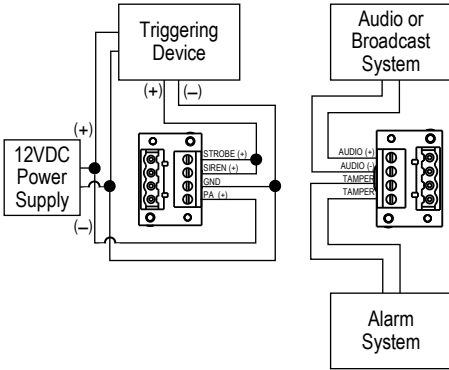
Triggering both siren and strobe* together (also showing audio input)
