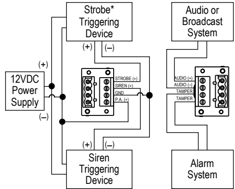
Siren and strobe* triggered by separate devices (also showing audio input)
