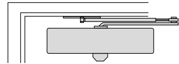
Parallel Arm
