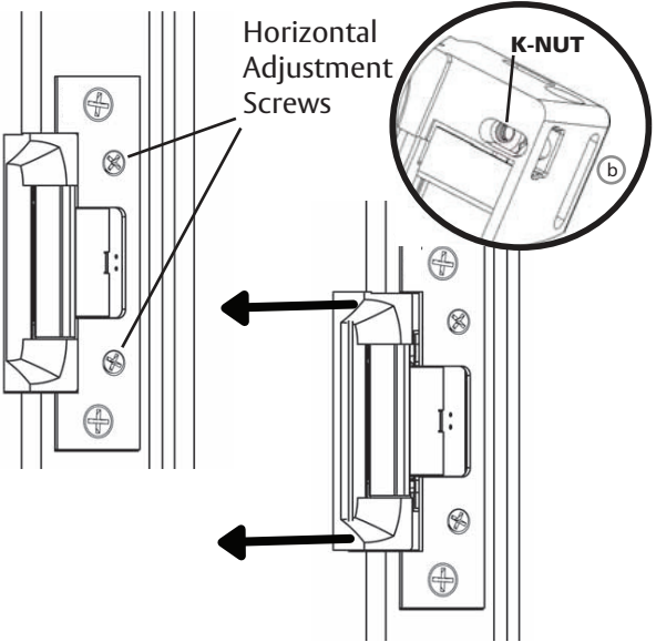
Diagram 6: Horizontal Adjustment
