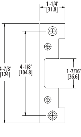
501 Faceplate Option (4-7/8" x 1-1/4"), Square Corners and Flat Faceplate Used with cylindrical locksets in ANSI metal jambs
