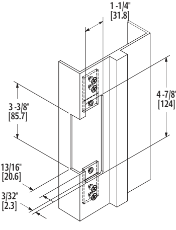
501A Faceplate Option (4-7/8" x 1-1/4"), Radius Corners and Flat Faceplate Used with cylindrical locksets or spring latches in aluminum frames
