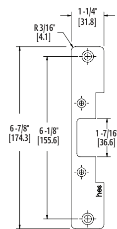
503 Faceplate Option (6-7/8" x 1-1/4"), Radius Corners and Flat Faceplate Used with cylindrical locksets or spring latches in aluminum frames
