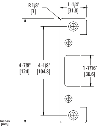
501A Faceplate Option (4-7/8" x 1-1/4"), Radius Corners and Flat Faceplate Used with cylindrical locksets or spring latches in aluminum frames
