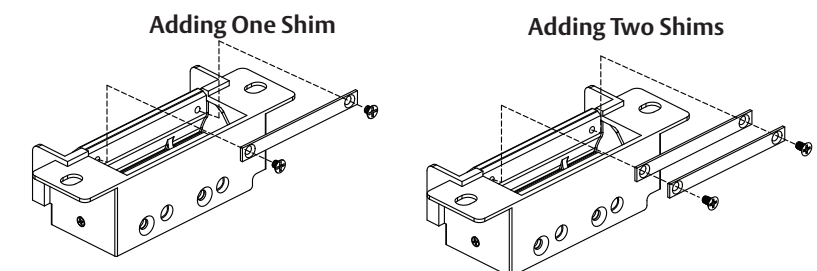
Figure 6: Horizontal Adjustment
