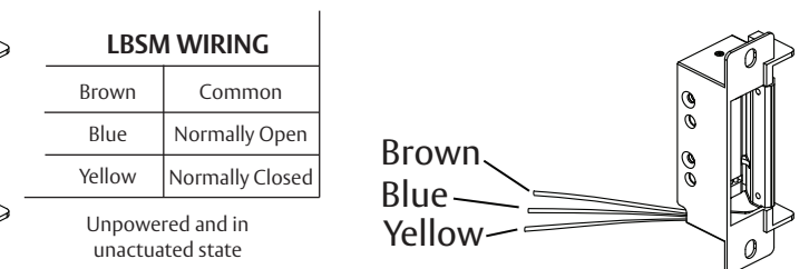
Figure 3: Strike Monitor
