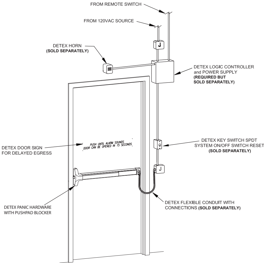
Typical Application - Delayed Egress with Access Control
