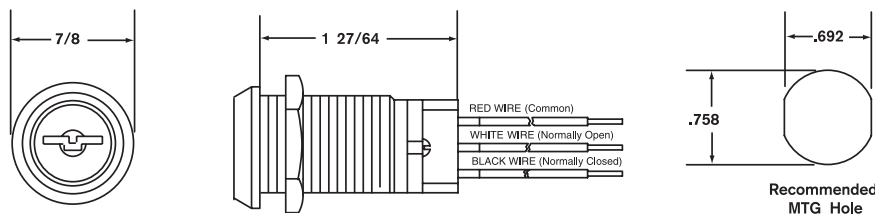
Double Bitted Switch Locks — SPDT
