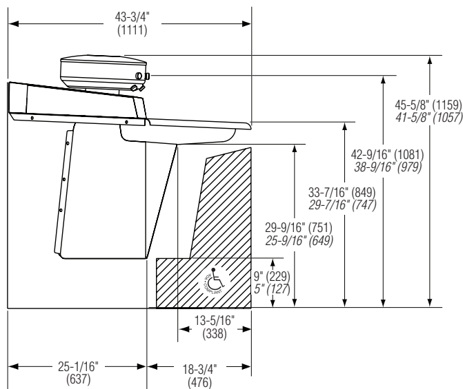
Wall-Mounted With Hand Control
