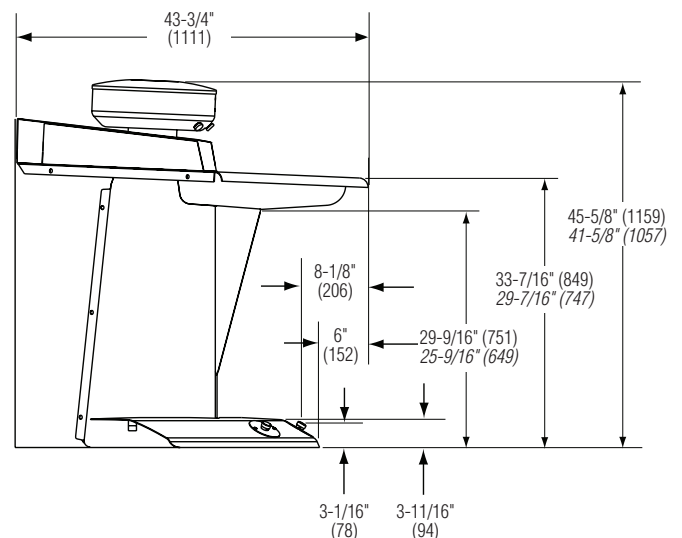
Wall-Mounted With Hand Control
