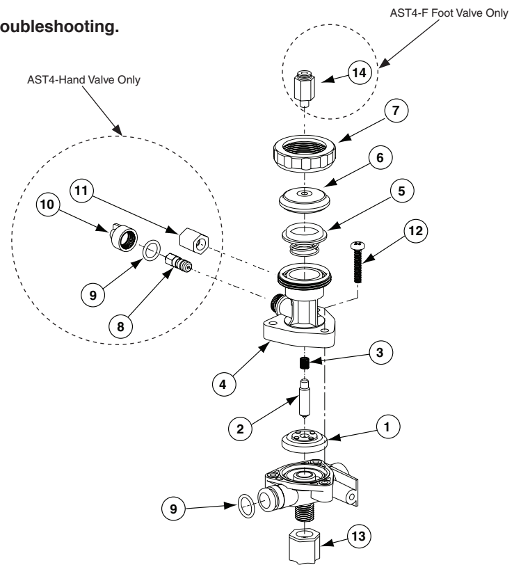
AST4-Hand Valve, AST4-F Foot Valve
