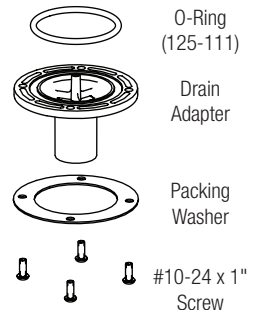
Drain Adapter Prepack (S45-2480)
