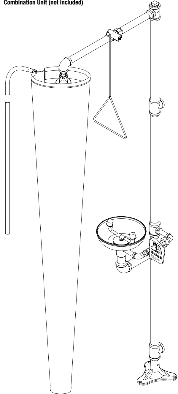
Drench Shower Tester shown with Bradley Combination Unit (not included)
