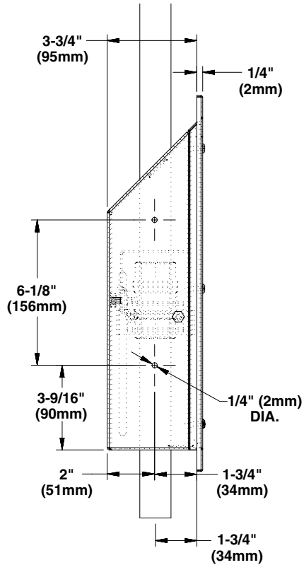
S19-125BF Cabinet Side View
