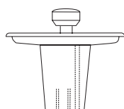
Type A Off-line vent (P-Trap supplied by Installer.)
