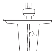
Type B Centrally rising vent - (P-Trap furnished) Use for units with paper down dispensers and/ or shrouds.
