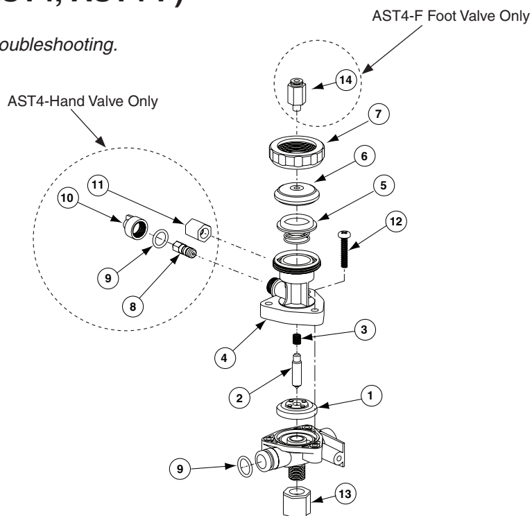
AST4-Hand Valve, AST4-F Foot Valve
