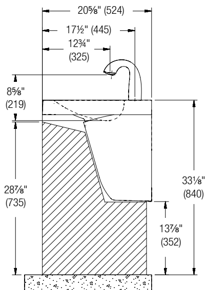
OBC Height – Verge Faucet
