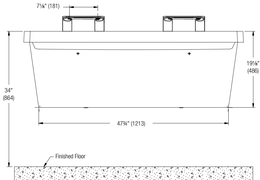
Front View (shown with WBD1)
