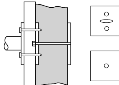
Back Anchor Plate
